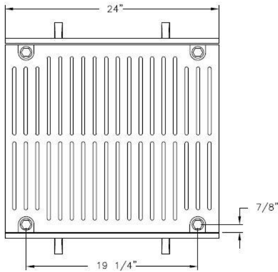
GRATE TOP VIEW
