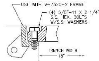
BOLT DOWN DETAIL
